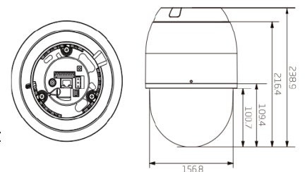
820 (Outdoor Model)
