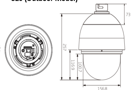
820 (Outdoor Model)
